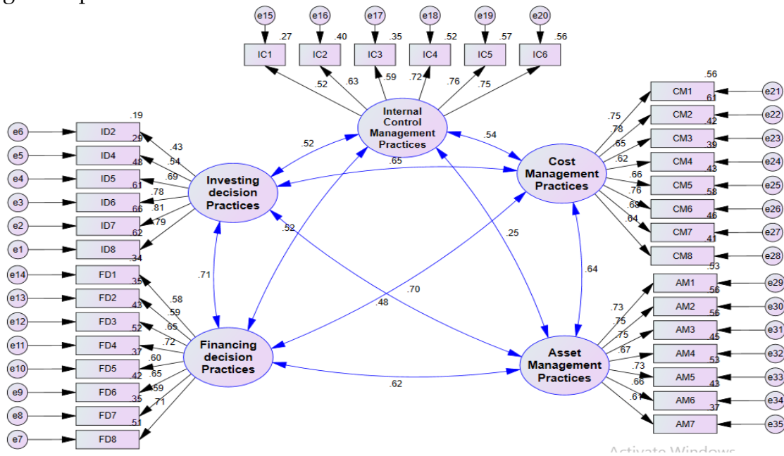
Figure 1. CFA Source: AMOS Output (2023)
