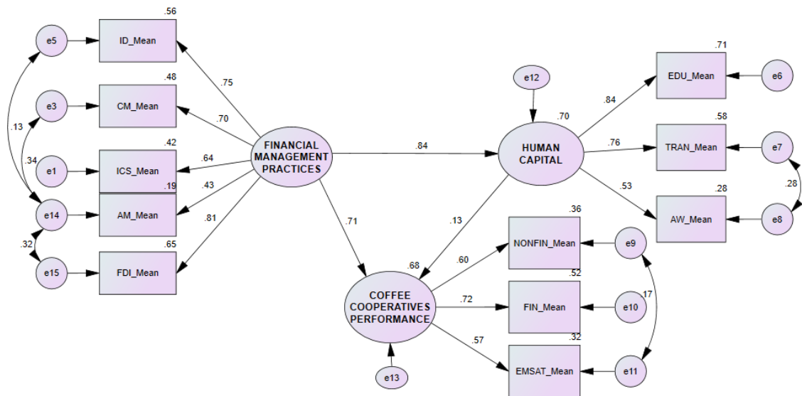
Figure 2. Structure Equation Modeling Source: AMOS Output (2023)
