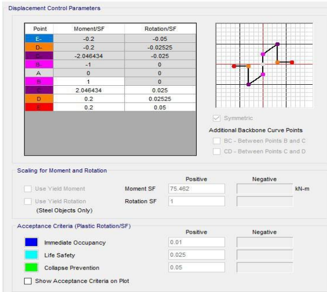
Figure 5. Assigned hinges properties according to FEMA-356
