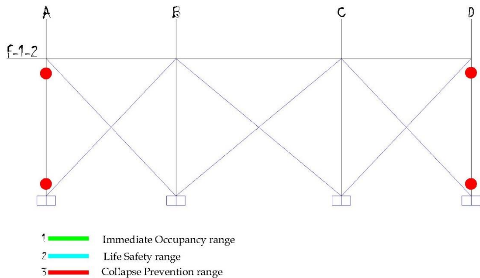
Figure 12. Plastic hinges creation as the result of pushover in Y direction (Step-6, 13mm of displacement)
