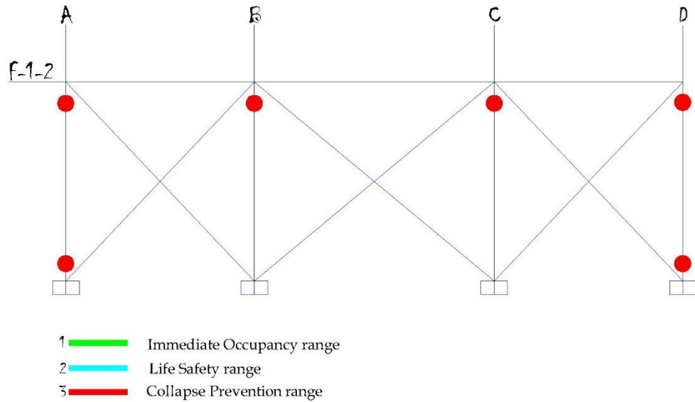
Figure 14. Plastic hinges creation as the result of pushover in Y direction (Step-10, 20mm of displacement)
