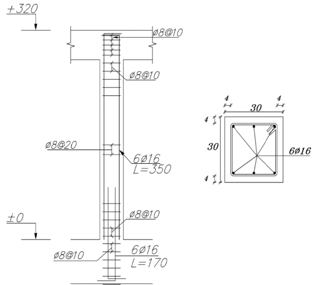
Figure 4. Column detail of existing structure
